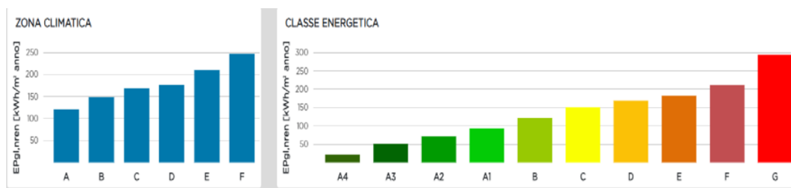
Figure 2 - Residential Buildings - Average of primary energy demands for climate zone (zona climatica) and EPC label (classe energetica) from SIAPE portal
